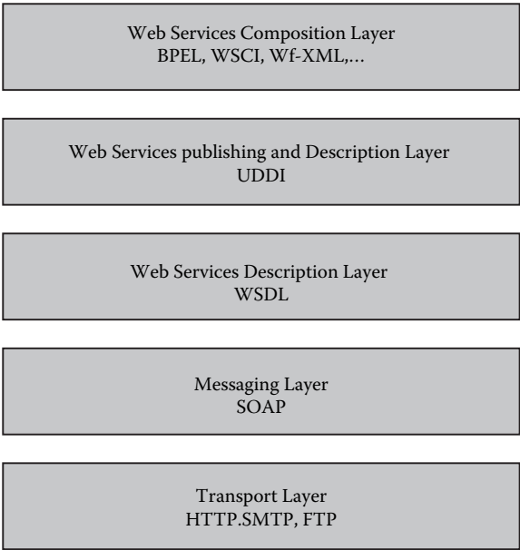
Figure 9.4 Web Services Stack.
