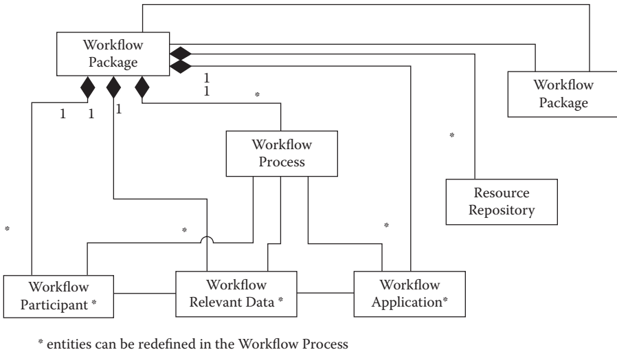
Figure 9.1 XPDL Meta-Model. (WfMC. 2002. Workflow Process Definition Interface — XML Process Definition Language. Document Number WfMC-TC-1025. p. 13. copyright©2002 Workflow Management Coalition.)
