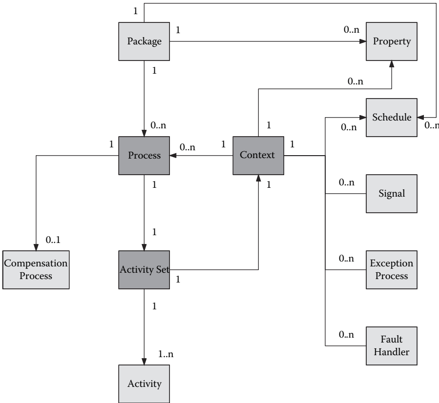
Figure 9.2 BPML Meta-Model.
