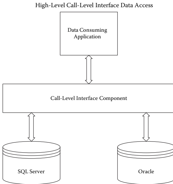
Figure 4.1 Overview of database access using CLI.
