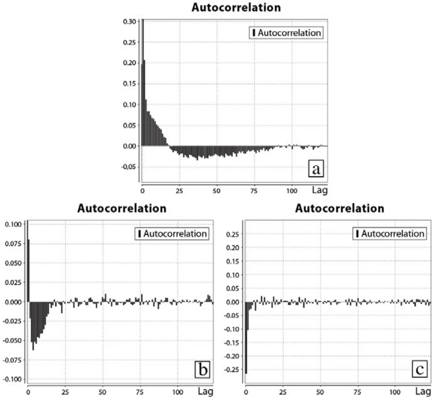
Fig. 4: Autocorrelation functions depending on deviation factor v (a) v=0.025 , (b) v=0.35 , (c) v=1
