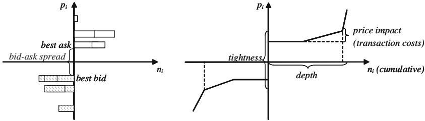
Fig. 1: Order book and liquidity characteristics representation
