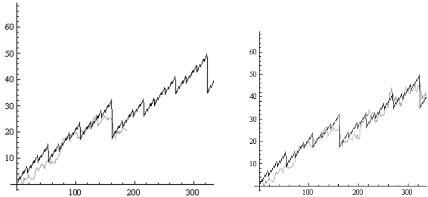
Fig. 7: IBM stock price in annual time frame (01.07.06-01.04.08)
