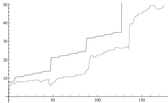
Fig. 5: Supercritical wave (third Level of Fractal) for D<1 , p=3 . This type of wave is not presented in the Elliott theory.
