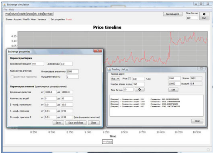
Fig. 1: General view of the developed application “Exchange simulator”
