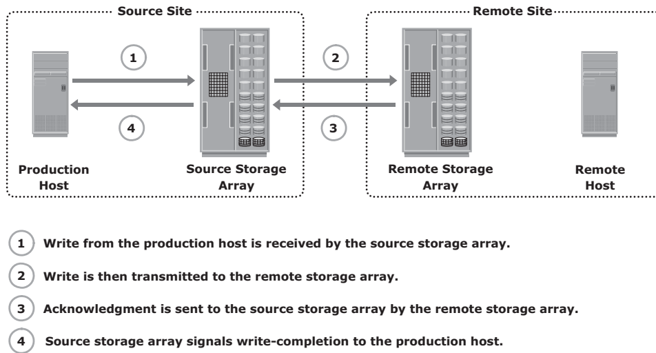
Figure 12-7: Array-based synchronous remote replication
