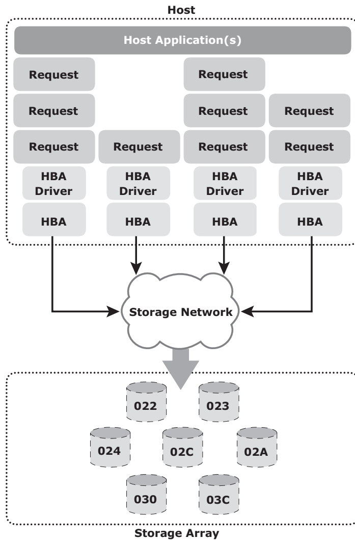
Figure 9-7: I/O without PowerPath
