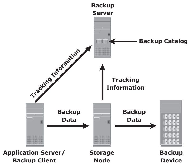
Figure 10-4: Backup architecture
